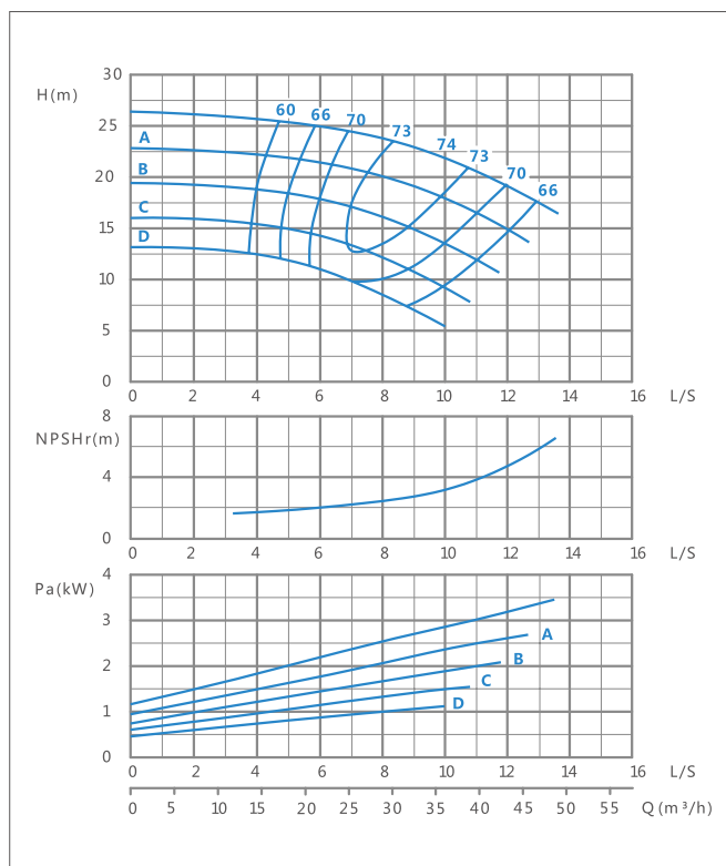
XA(T) 40/20-2900r/min Performance curve
