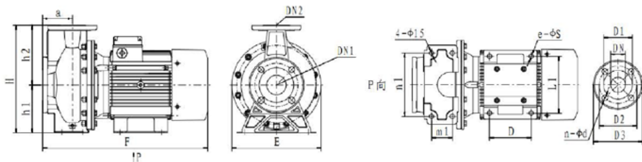
Flange Dimensions
