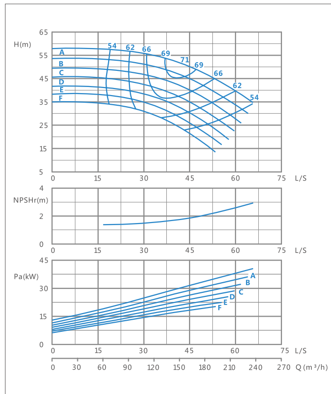
XA(T) 100/40-1450r/min Performance curve
