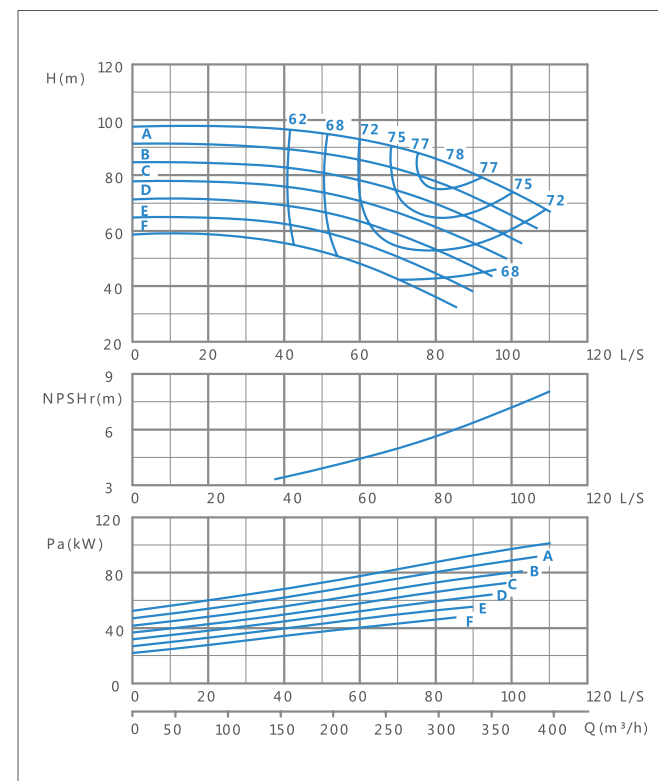
XA(T) 32/13-1450r/min Performance curve
