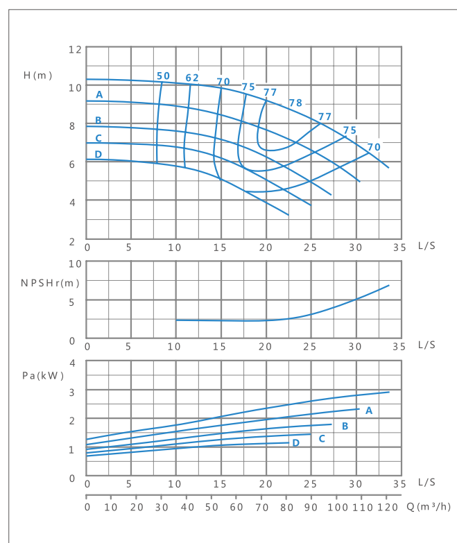
XA(T) 80/16-1450r/min Performance curve
