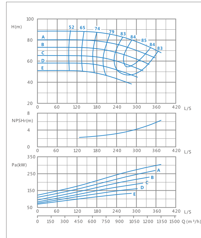
XA250/50-1450r/min Performance curve
