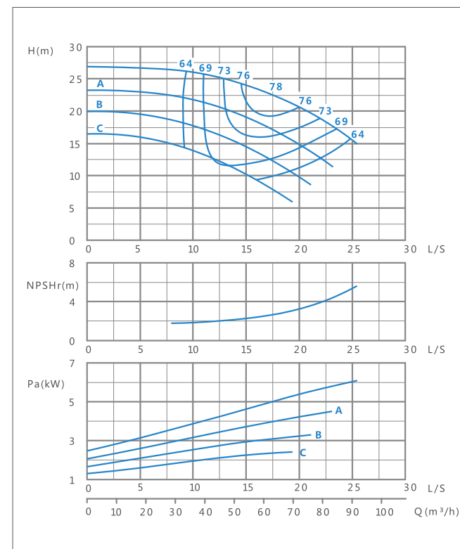
XA(T) 50/20-2900r/min Performance curve
