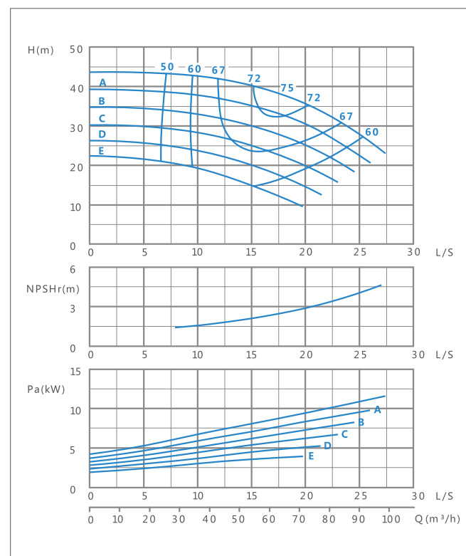
XA(T) 50/16-2900r/min Performance curve
