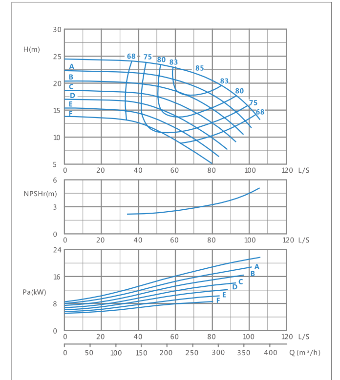
XA(T) 125/40-1450r/min Performance curve
