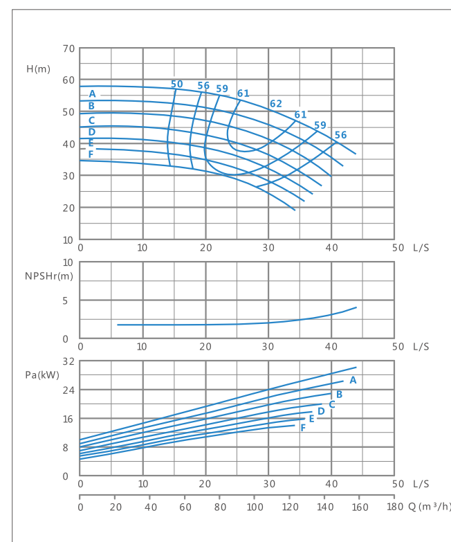
XA(T) 80/40-1450r/min Performance curve
