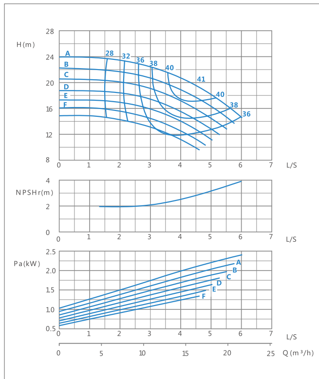
XA(T) 32/26-1450r/min Performance curve
