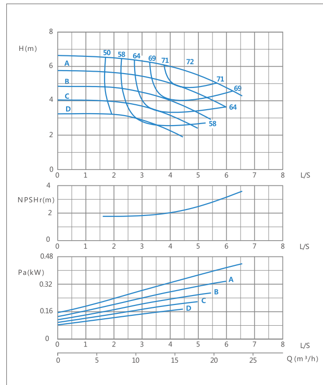
XA(T) 40/13-1450r/min Performance curve
