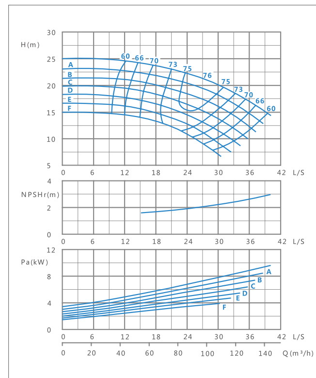
XA(T) 80/40-1450r/min Performance curve
