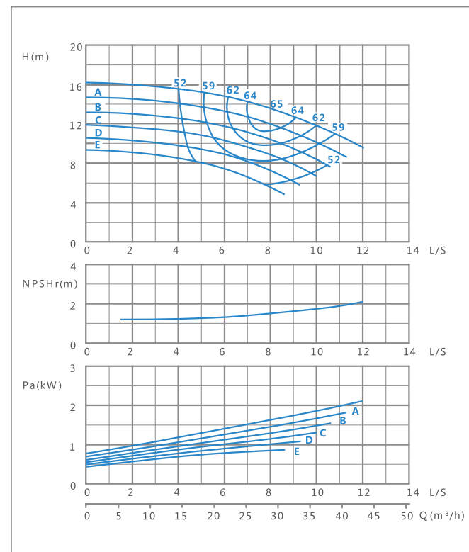
XA(T) 50/20-1450r/min Performance curve
