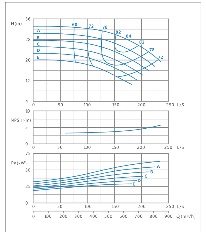
XA200/32-1450r/min Performance curve
