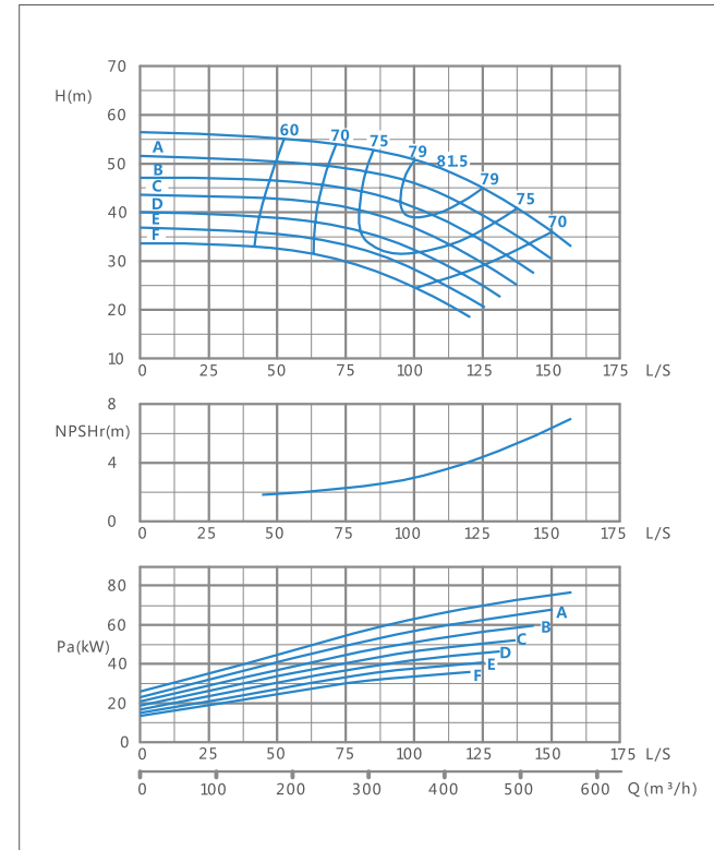
XA200/26-1450r/min Performance curve
