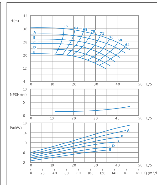
XA(T) 100/16-1450r/min Performance curve
