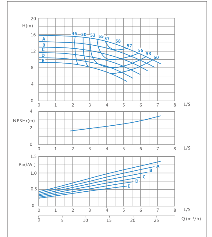
XA(T) 40/32-1450r/min Performance curve
