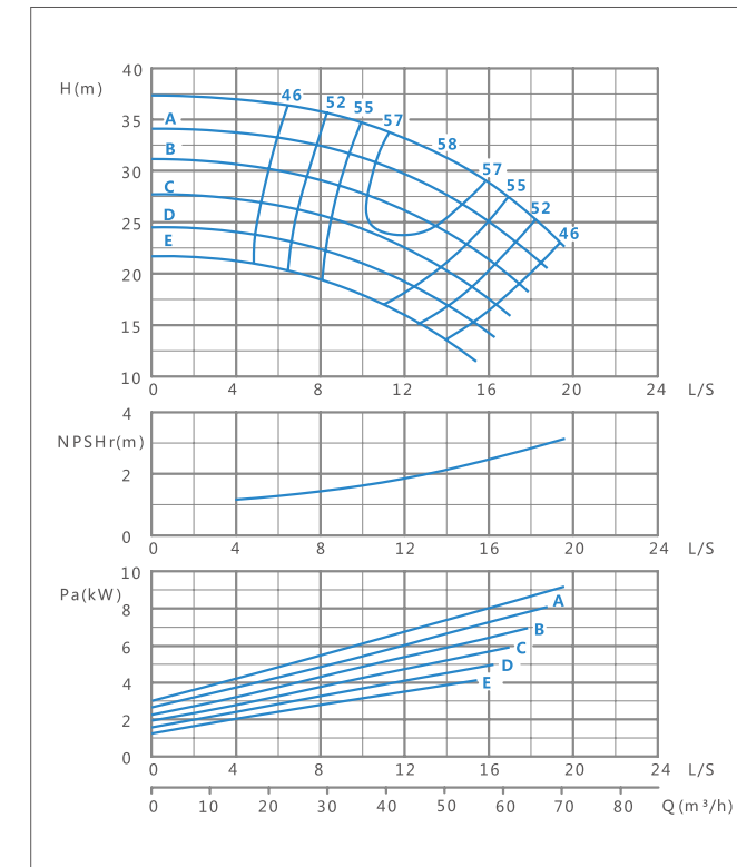
XA(T) 65/16-1450r/min Performance curve
