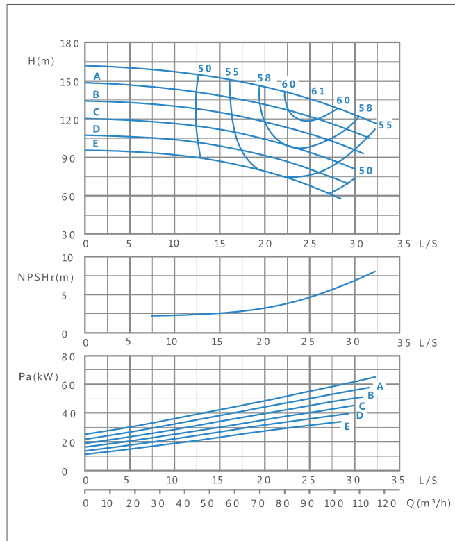
XA(T) 65/16-2900r/min Performance curve
