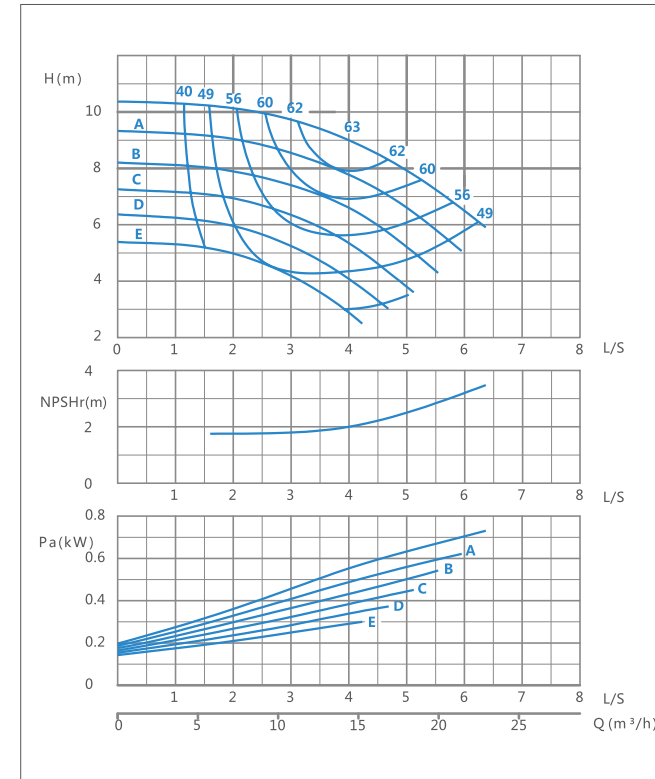
XA(T) 40/26-1450r/min Performance curve
