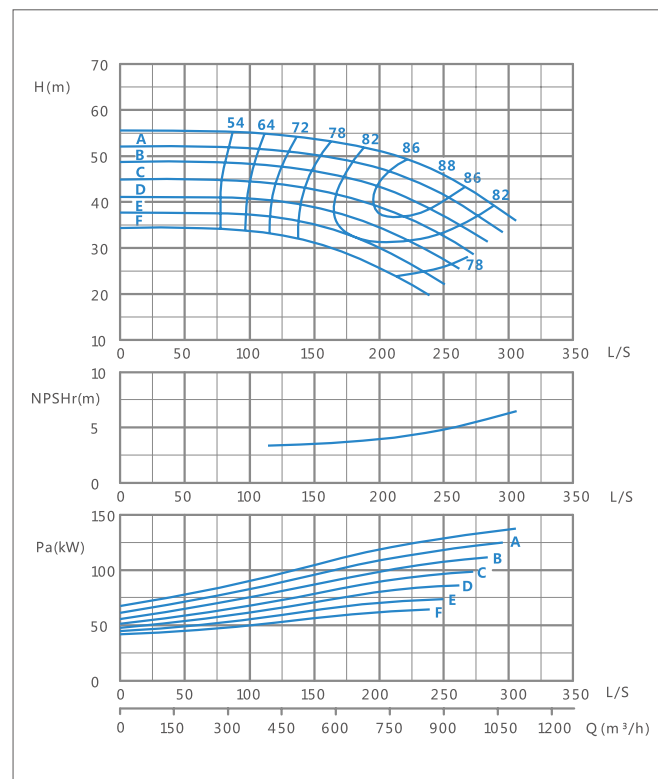
XA250/40-1450r/min Performance curve
