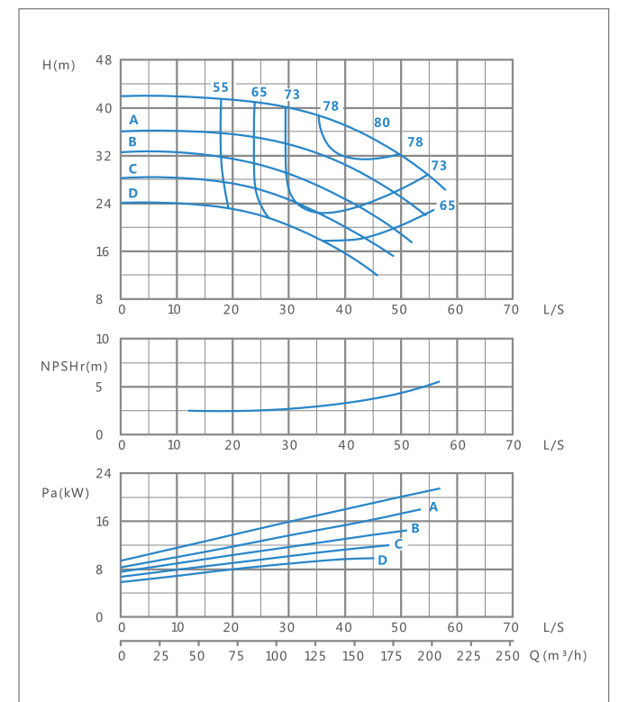
XA(T) 80/16-2900r/min Performance curve
