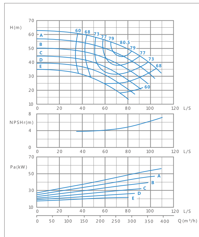
XA(T) 125/20-2900r/min Performance curve
