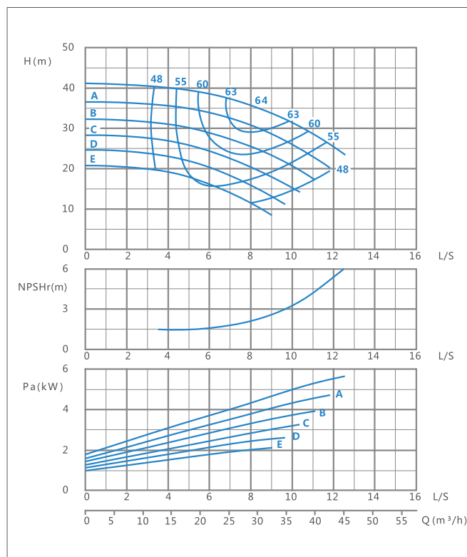
XA(T) 40/26-2900r/min Performance curve
