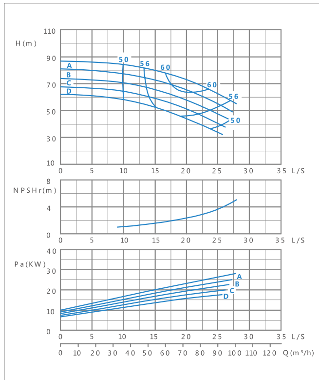
XA(T) 65/13-2900r/min Performance curve
