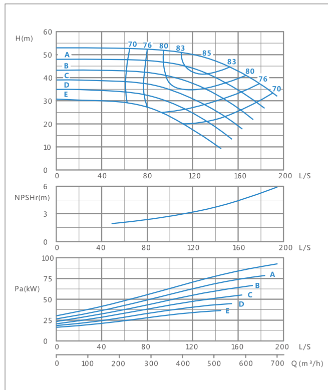
XA(T) 150/32-1450r/min Performance curve
