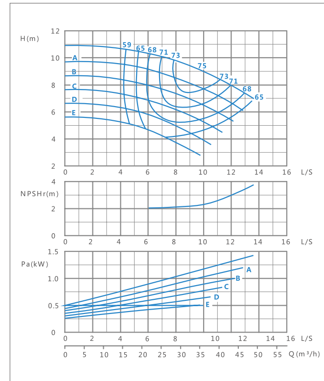
XA(T) 50/26-1450r/min Performance curve
