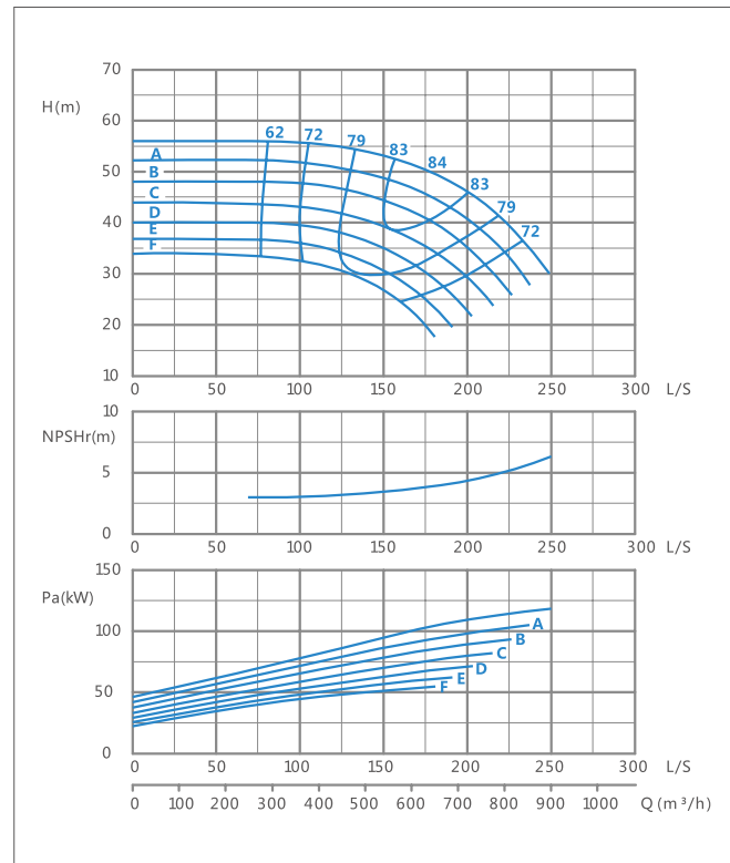
XA250/32-1450r/min Performance curve
