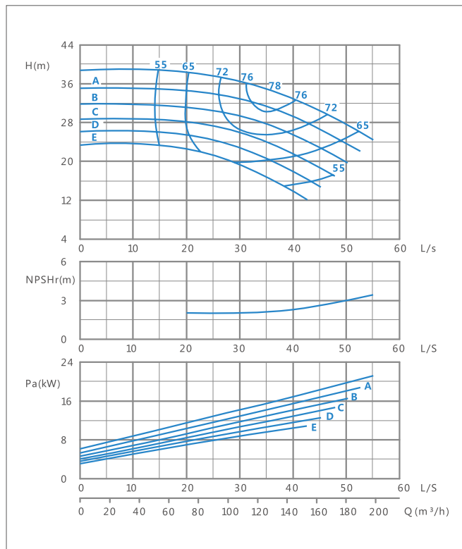
XA(T) 100/32-1450r/min Performance curve
