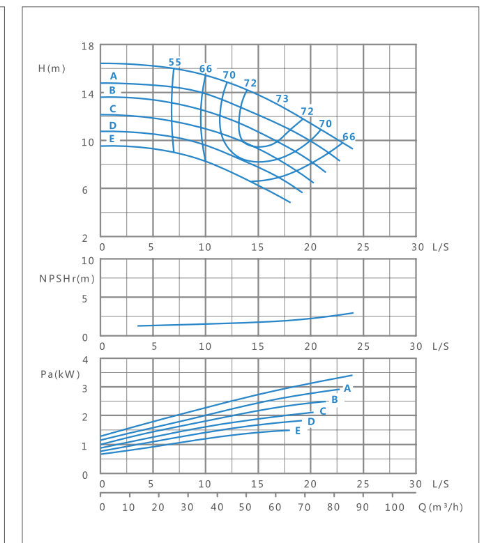
XA(T) 65/20-1450r/min Performance curve
