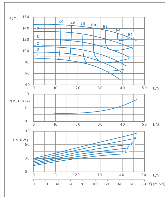
XA(T) 65/32-2900r/min Performance curve
