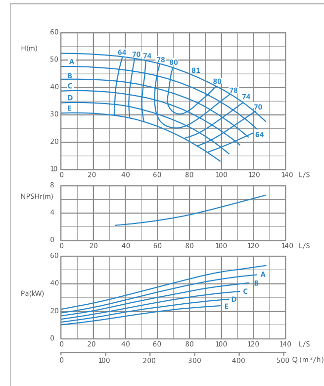
XA(T) 125/32-1450r/min Performance curve
