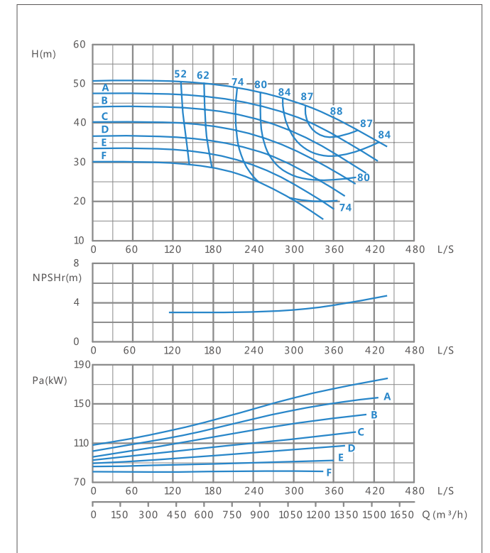
XA300/40-1450r/min Performance curve
