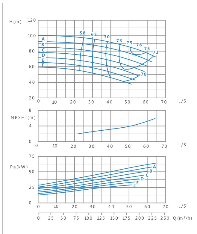
XA(T) 100/16-2900r/min Performance curve
