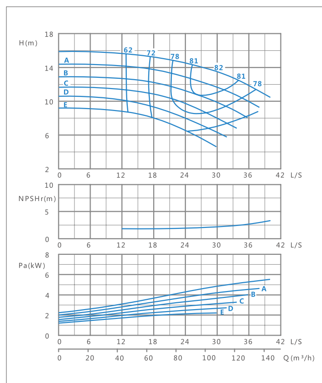
XA(T) 80/20-1450r/min Performance curve
