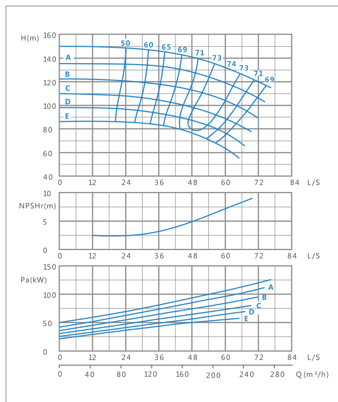
XA(T) 80/32-2900r/min Performance curve
