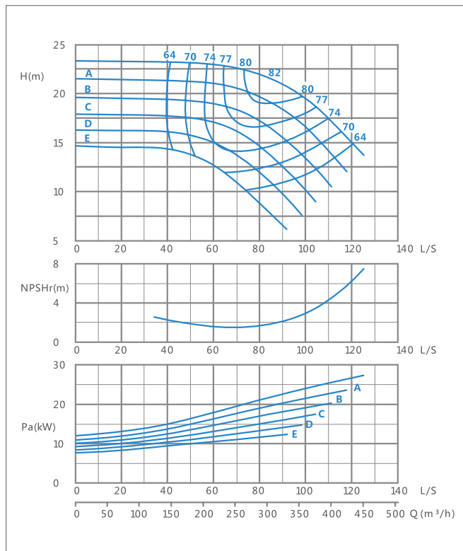
XA(T) 150/26-1450r/min Performance curve
