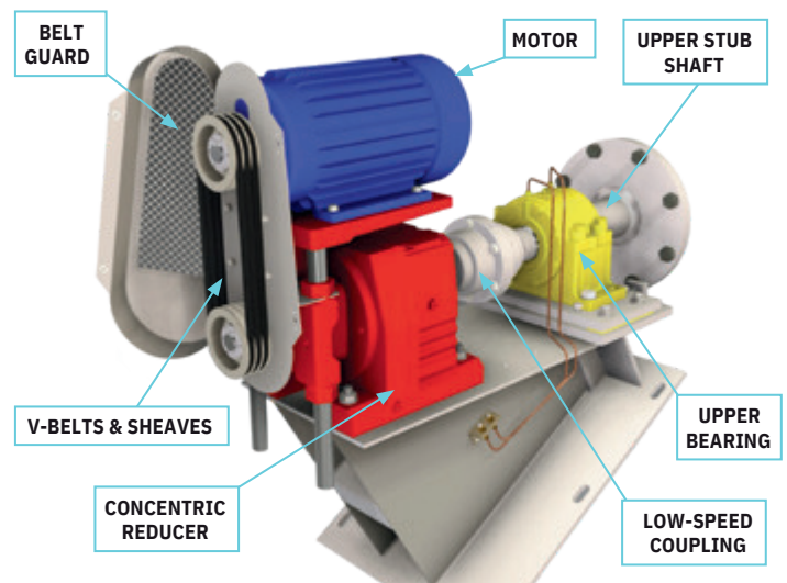
Concentric Drive Assembly
