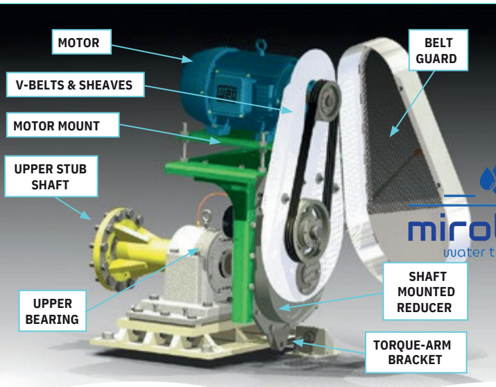
Shaft-Mounted Drive Assembly
