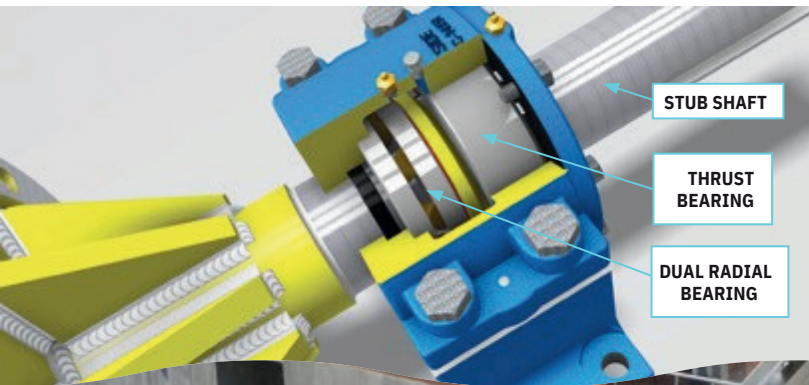
Upper Bearing Assembly
