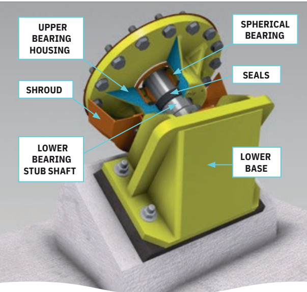
Sealed Type "E" Lower Bearing Assembly
