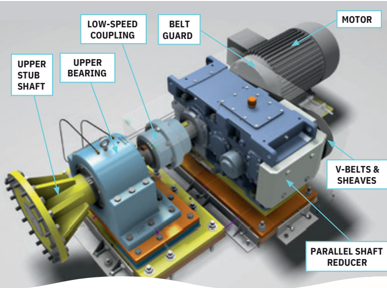
Parallel-Shaft Drive Assembly
